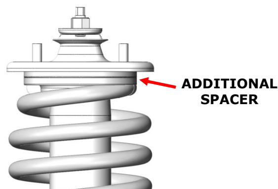
Figure B Rear Strut with additional Spacer Fitted
