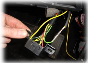
Coil spring harness wire attached to (green) vehicle harness wire previously removed from diagnostics connector
